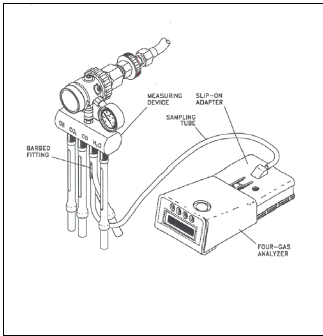
Figure 6, PHD Ultra Four Gas Analyzer Connection to Air Test Kit
