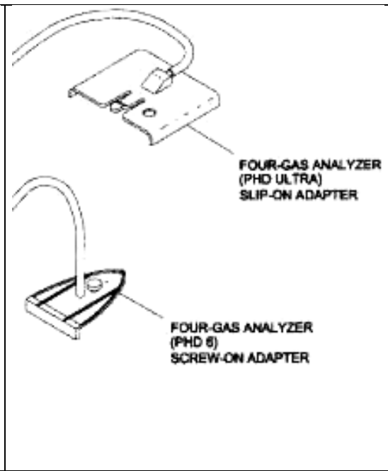
Figure 7, Air Test Kit Connections to PHD Ultra or PHD6 Gas Analyzers
